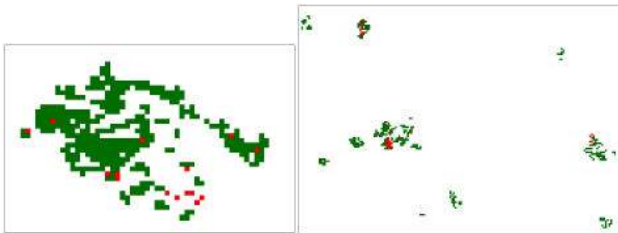
Figure 3 and 4. ATSR hotspots (red) superimposed over AVHRR hotspots (green) for large burn in Northwest Territories (see region A on Figure 1) and in Manitoba (see region B)
