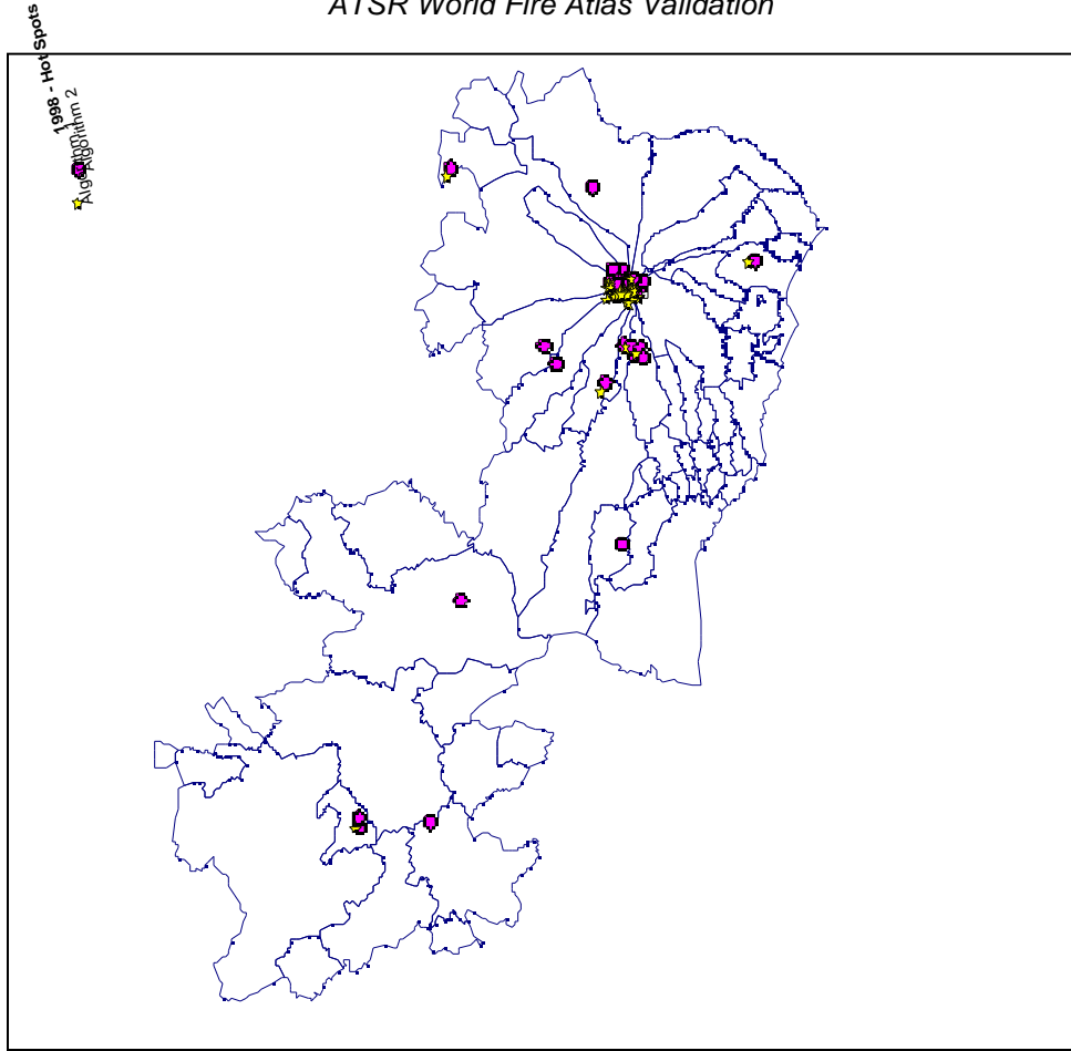
Fig. 1 – Hot Spots for 1998 with Algorithm 1 and 2
