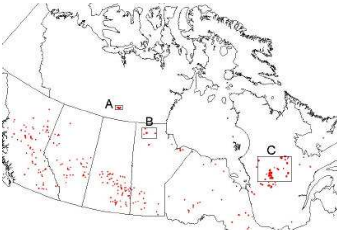
Figure 1. ATSR hotspots detected over Canada between April-October, 1997
