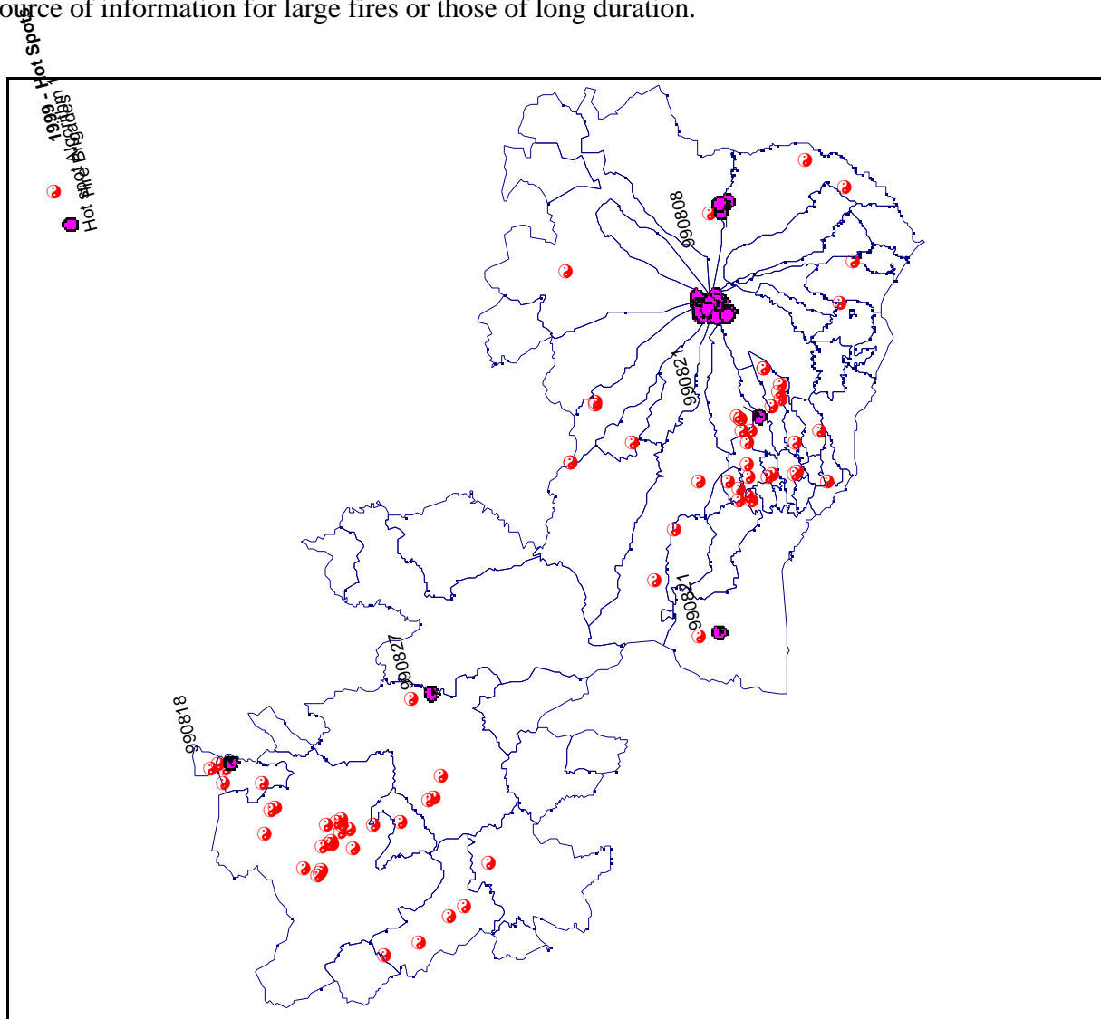
Fig 3 – Hot Spots and Fire Brigade logs – August 1999
