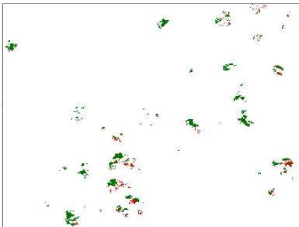
Figure 5. ATSR hotspots (red) superimposed over AVHRR hotspots (green) for active fire region in Quebec (see region C on Figure1)
